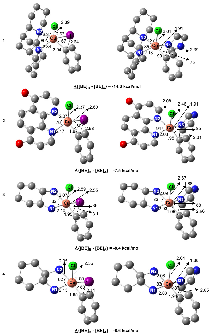
Figure 2. 3D representations of DFT optimized geometries (with BLYP functionals) along with important geometric parameters for Cu(III) intermediates (A and B) derived from (1) (–)-sparteine, (2) 4,7-dihydroxy-1,10-phenanthroline, (3) trans -1,2-cyclohexyldiamine ( chair ), and (4) trans -1,2-cyclohexyldiamine ( boat ) ligands. Hydrogen atoms are omitted for clarity. See Supplementary data for PW91 functional optimized DFT geometries.
