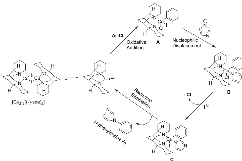
Figure 1. Proposed pentacoordinate Cu(III) intermediates in the mechanistic scheme for bis( \mu -iodo)bis((–)-sparteine)dicopper(I) catalyzed N-arylation of imidazole using aryl chlorides.
